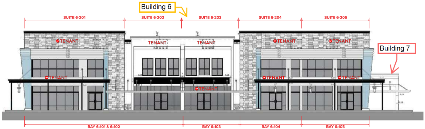
EAST ELEVATION (FRONT) 1/16" = 1'-0"
