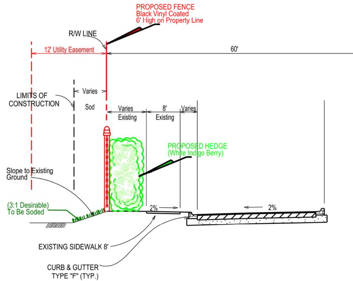
TYPICAL SECTION GREENVIEW SHORES BLVD. NTS
