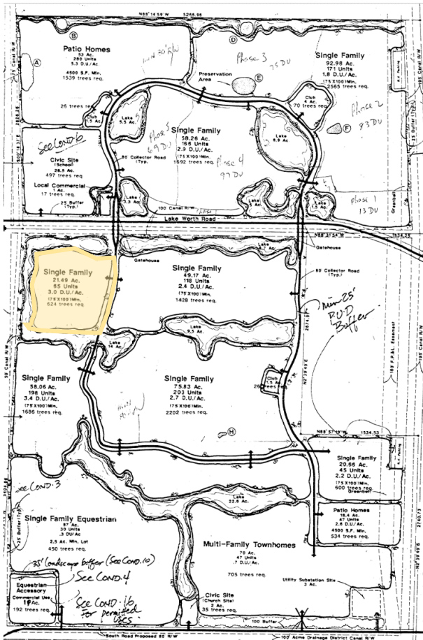
Figure 2: 1984 Approved Orange Point PUD Master Plan
