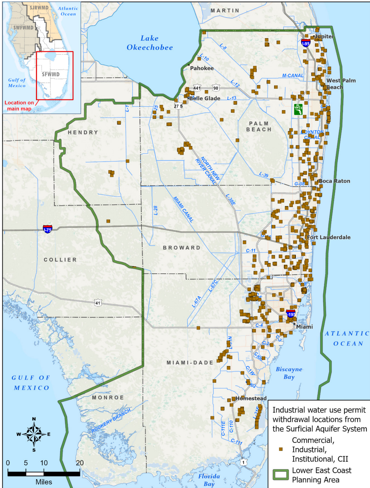
Figure 5-10. Commercial/Industrial/Institutional water use permit withdrawal locations from the surficial aquifer system within the LEC Planning Area.
