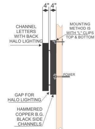
SIDE VIEW NORTH ELEVATION
