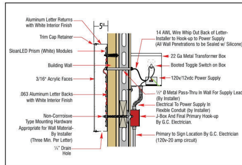
SECTION DETAIL - LED ILLUMINATED WALL LETTERS
