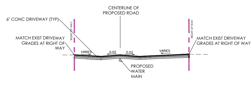
CROSS SECTION AT HIGH POINT
