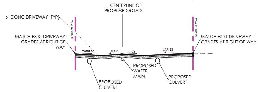
CROSS SECTION AT LOW POINT
