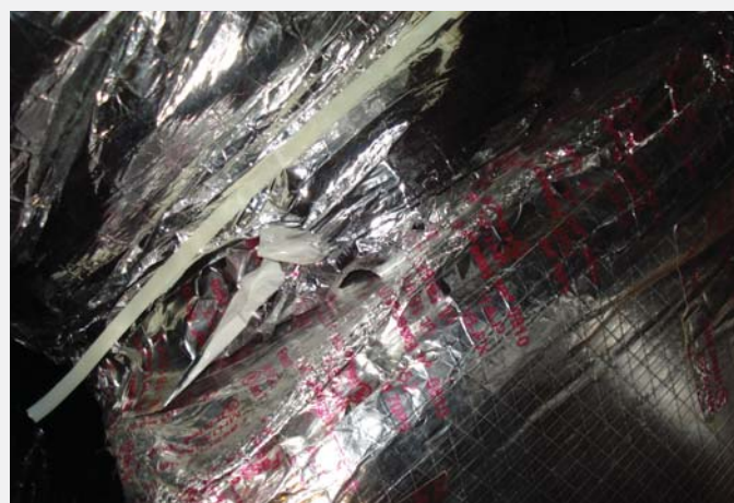
Flex duct not installed properly FBC 5th Edition Mechanical 603.9/Residential M1601.4.2
