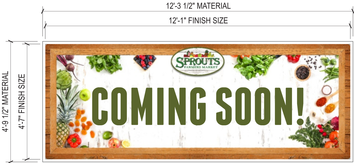
MFG. S/F DIGITAL PRINTED BANNER SCALE: 1/2" = 1'-0" HEMMED AND GROMMETED AT CORNERS & CENTER S/F BANNER MATERIAL - 13 OZ ARLON GLOSS WHITE
