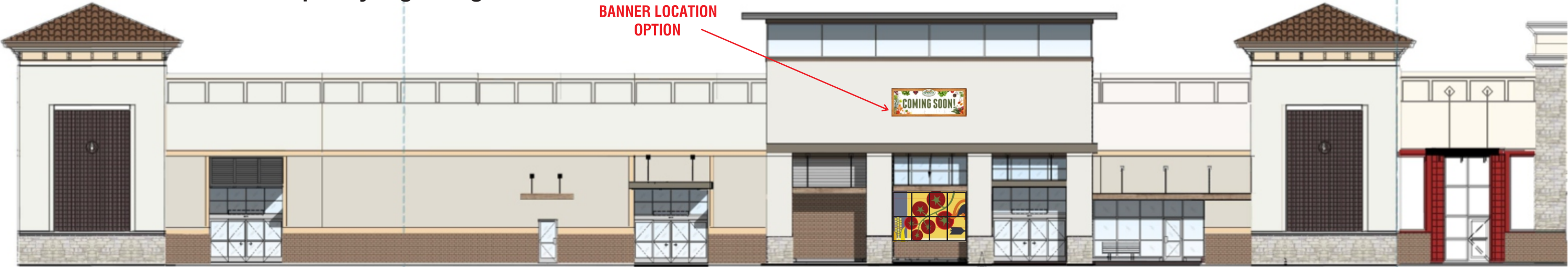
Front (West) Elevation Scale: 1/16" = 1'-0"
