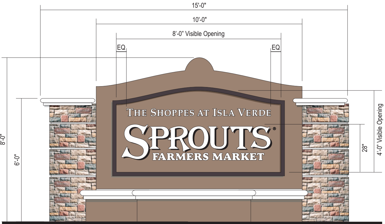
MONUMENT SIGN SHOWING PROPOSED LETTERS : 3/8" = 1'-0"
